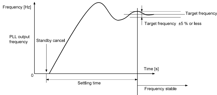
Figure 24 Definition of settling time
