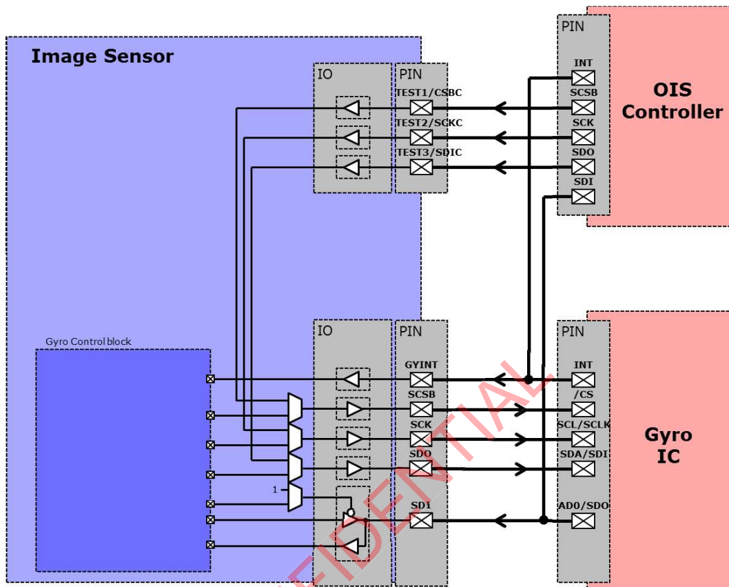
Figure 6 Connection diagram for OIS compatible system
