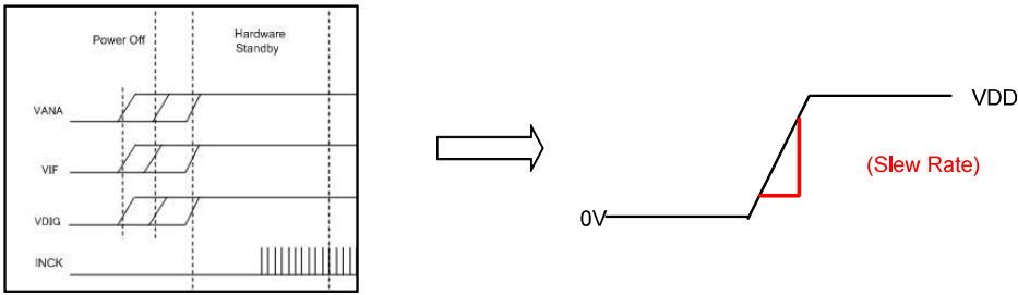
Figure 20 Power on slew rate
