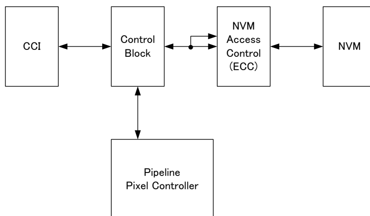
Fig. 33 Block Diagram
